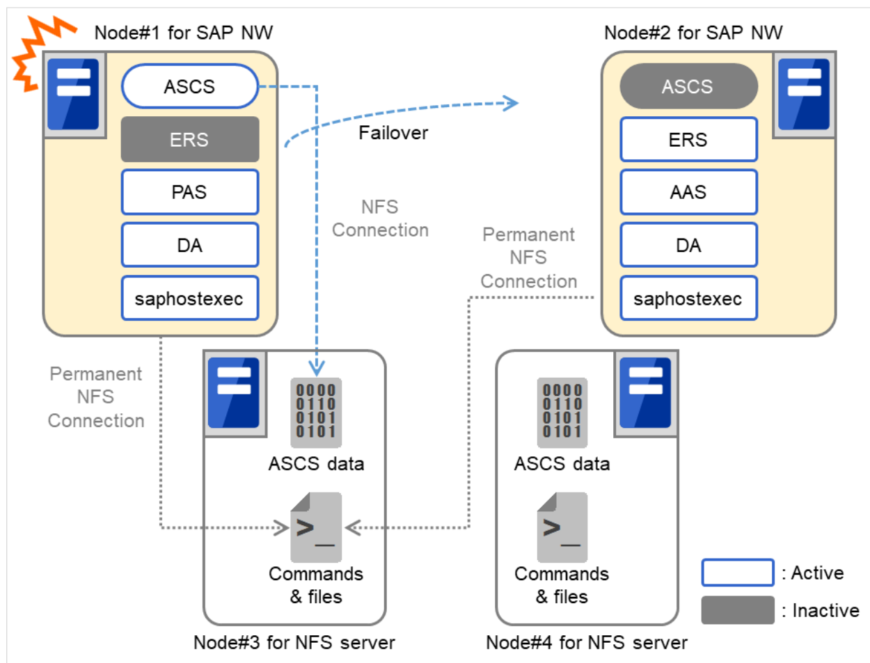
Fig. 3.3: System Configuration Using Two NFS Servers When a Failure Occurs in an SAP NW Server (1)
